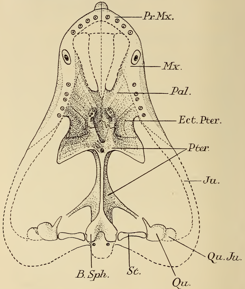
FIG. 15.— Arctognathus curvimola . Type, B.M.N.H., 47339. Ventral view of the skull, modified after Watson. \times \frac{2}{3} .
